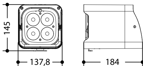
Technical drawing
